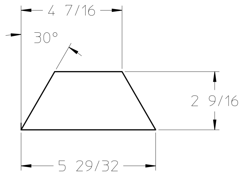
FRONT2 SCALE 1:2.5
